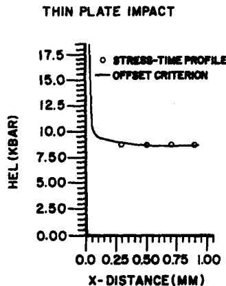
Fig. 11. Comparison of HEL from stress-time profiles and offset criterion in thin plate impact in 7039 aluminum.
