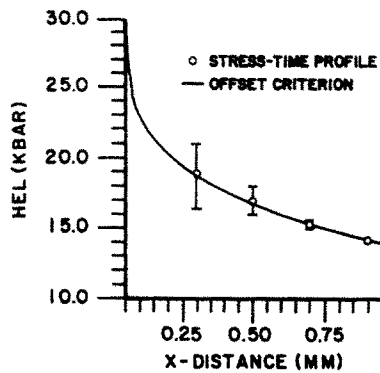
Fig. 12. Comparison of HEL from stress-time profiles and offset criterion in thin plate impact in C1008 steel.
